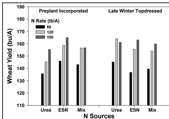
Figure 1. Three year average wheat yield as affected by fertilizer urea, ESN®, or a 50/50 mixture applied preplant or as a topdress in late winter at Parma.
